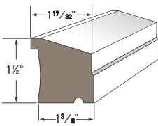
SUB SILL NOSE AZM-6933 Length: 16'
