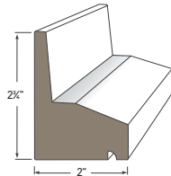
WATER TABLE AZM-6935 Length: 18'
