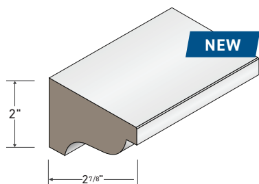
PEDIMENT CROWN MOULDING AZM-1882 Length: 12'
