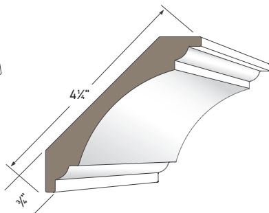
COVE MOULDING AZM-80 Length: 16'
