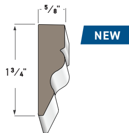
PANEL MOULD AZM-165 Length: 16'
