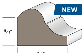
NOSE COVE AZM-7480 Length: 16'
