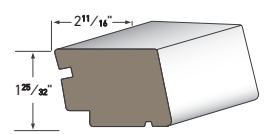
LARGE HISTORIC SILL AZM-7958 Length: 16'
