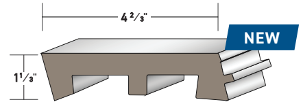
PCB SILL AZM-948 Length: 16'
